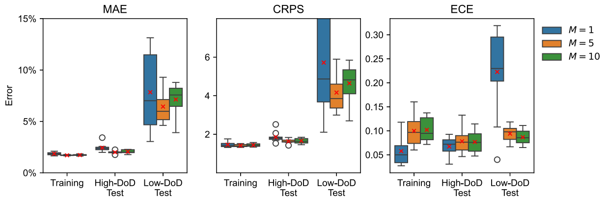
Fig. 9. Performance of end-to-end neural network ensembles (E2E-NNE) using different ensemble sizes ( M ). Each ensemble consists of M individual mean-variance networks.
