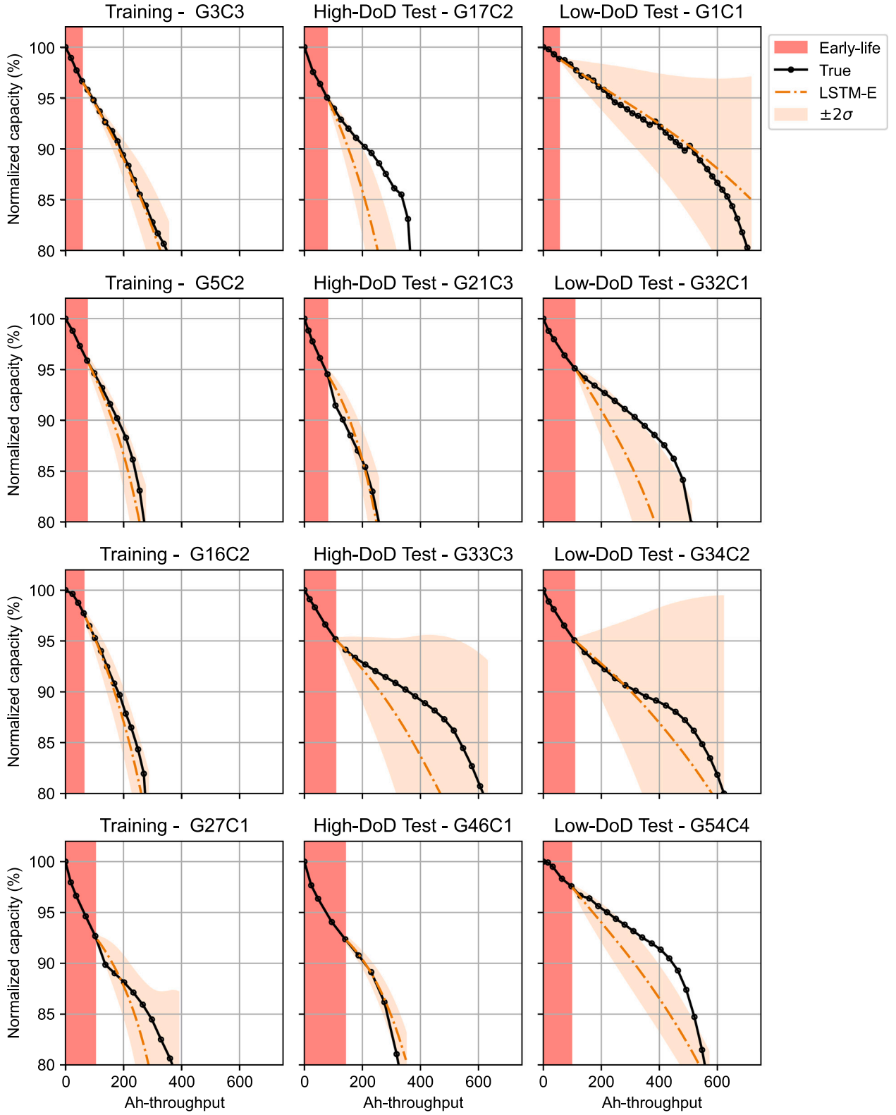
Fig. A.7. Predicted trajectories from LSTM-E method for selected cells in the public NCA dataset.
