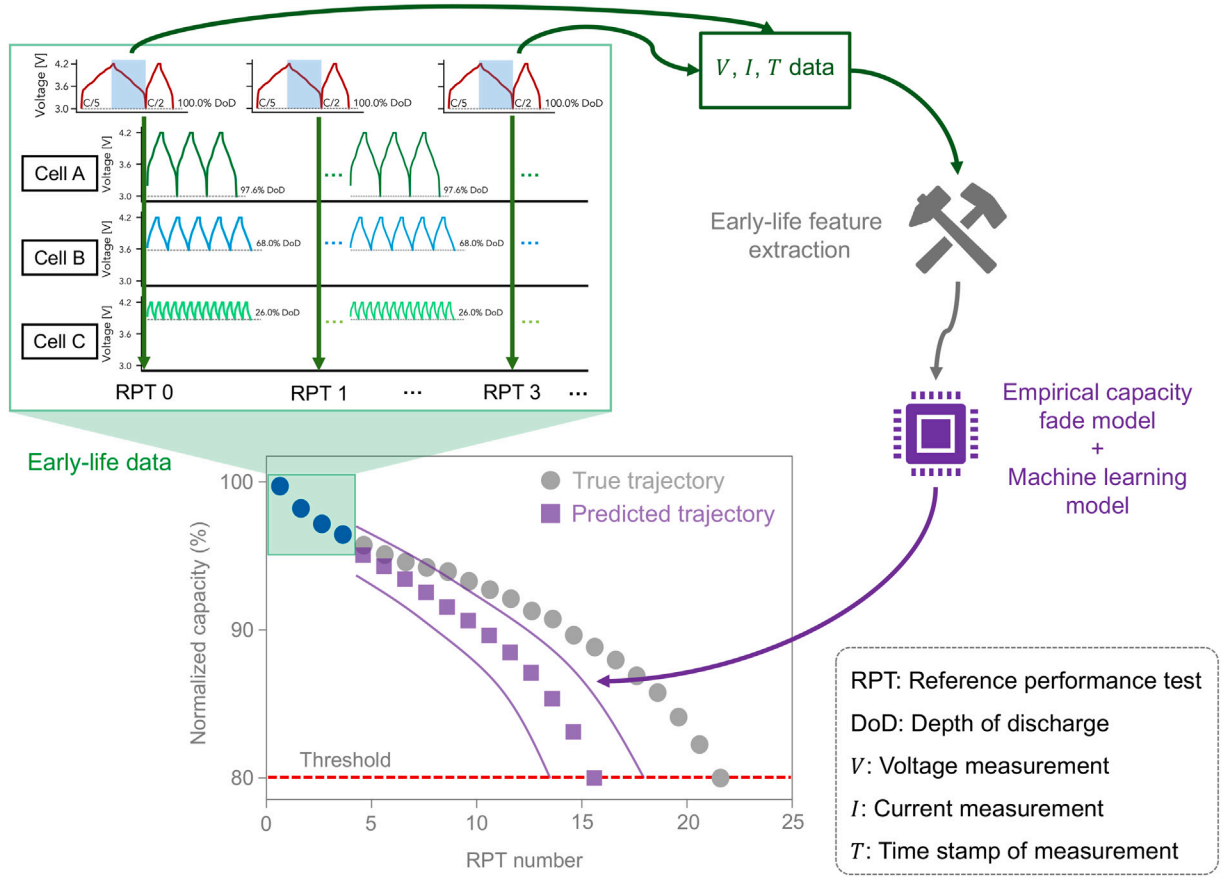
Fig. 2. An overview of the early trajectory prediction problem studied in this work.
