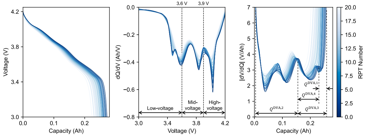
Fig. A.1. The evolution of capacity–voltage curves, incremental capacity curves, and differential voltage curves as the NMC cell ages.
