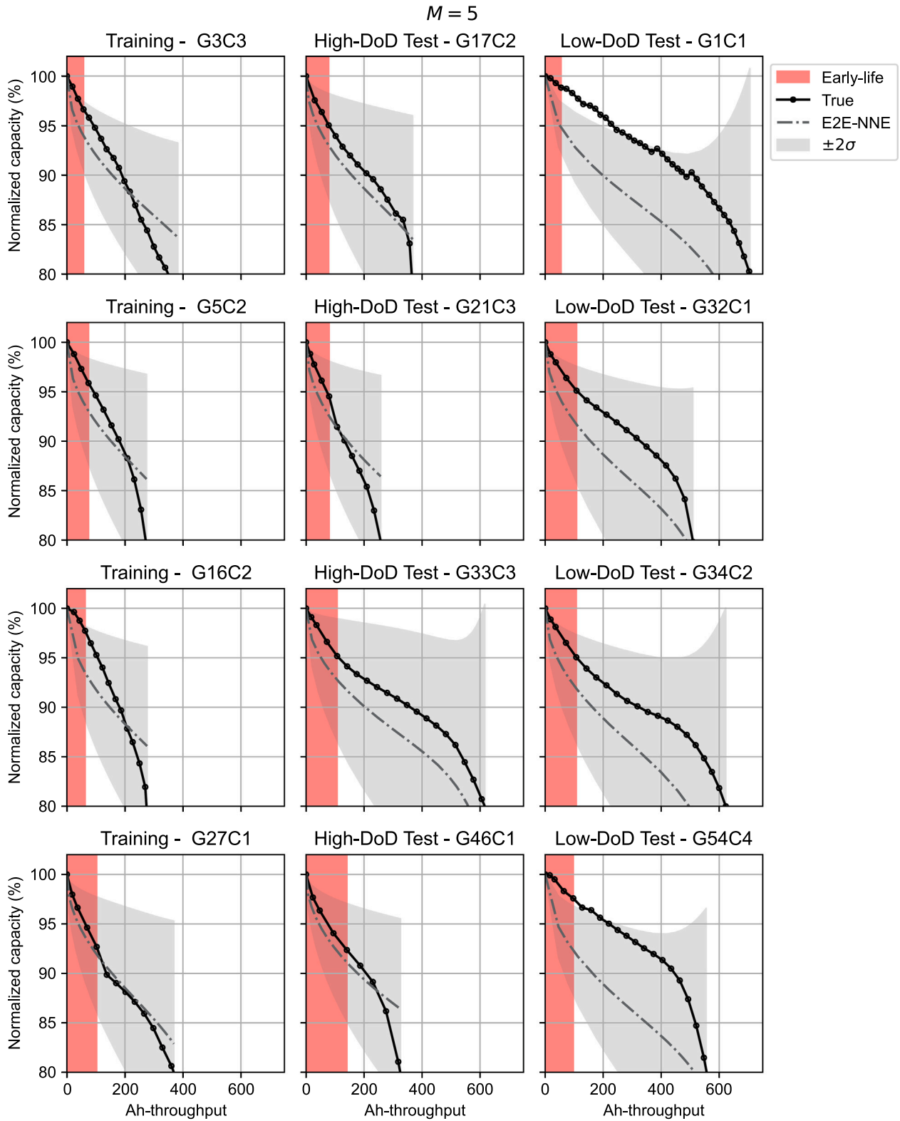
Fig. A.5. Predicted trajectories from E2E-NNE ( M = 5 ) for selected cells.
