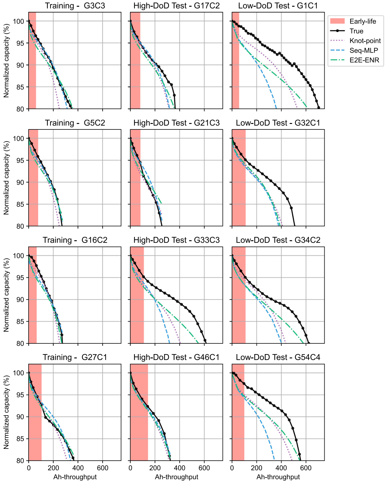
Fig. A.3. Predicted trajectories from selected deterministic methods for selected cells.
