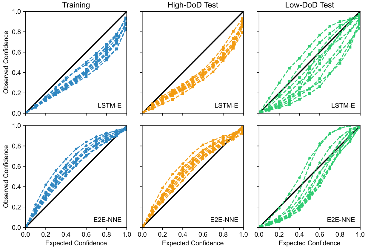
Fig. 14. Calibration curves of LSTM-E and E2E-NNE on the three subsets.
