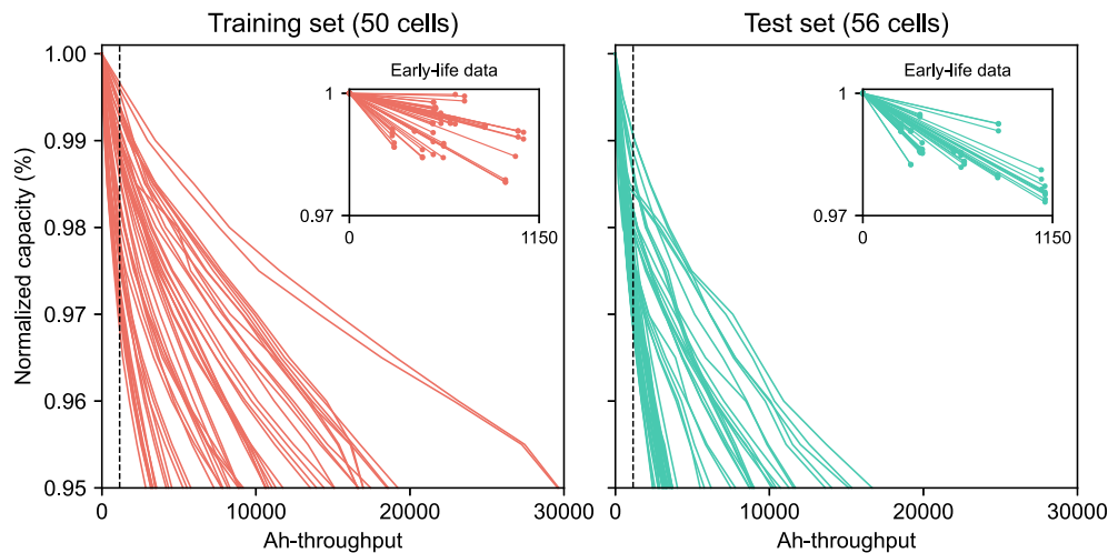
Fig. 15. Capacity trajectories of cells from the public NCA dataset after preprocessing. The black dashed line highlights the Ah-throughput value of 1150, indicating the threshold before which all early-life data are collected.
