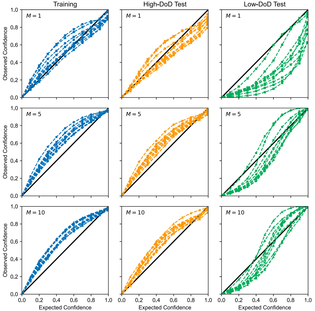
Fig. 10. Calibration curves for the E2E-NNE method with different numbers of individual models M on the three subsets.
