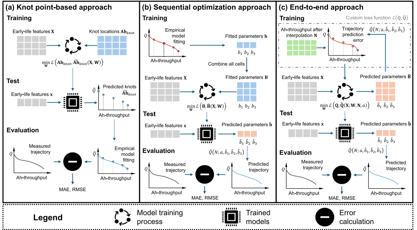
Fig. 5. Overview of capacity trajectory prediction approaches. (a) Knot point-based prediction of empirical model parameters; (b) sequential prediction of empirical model parameters; (c) end-to-end prediction of empirical model parameters.
