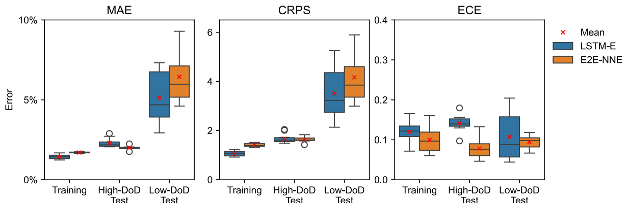
Fig. 13. Fold-to-fold performance variation of LSTM-E and E2E-NNE, evaluated by three metrics for probabilistic predictions.
