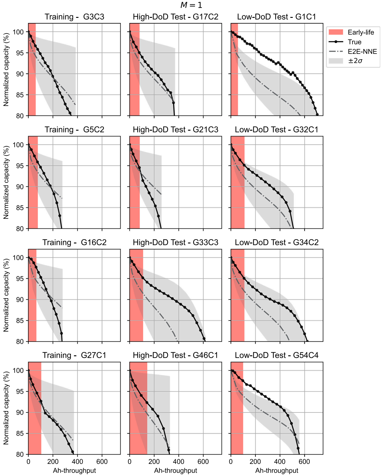
Fig. A.4. Predicted trajectories from E2E-NNE ( M = 1 ) for selected cells.
