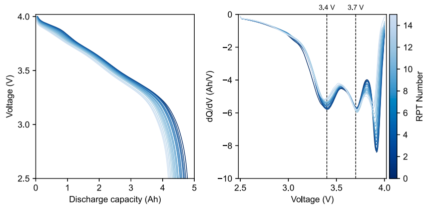
Fig. A.2. The evolution of capacity–voltage curves and incremental capacity curves as the NCA cell ages.
