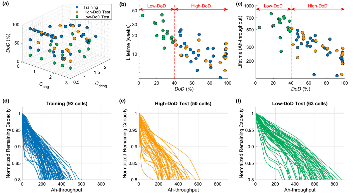
Fig. 4. Overview of the dataset partition. (a) Scatter plot of cycling conditions for each group, colored by its assigned subset after partitioning. (b) Group mean lifetime (in weeks) against DoD, measured by time on test. (c) Group mean lifetime against DoD, measured by total Ah-throughput. (d–f) Capacity trajectories for cells in three different subsets: (d) training set, (e) high-DoD test set, and (f) low-DoD test set.
