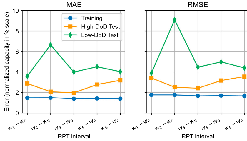
Fig. 11. Prediction performance of the E2E-ENR method with PCA features extracted from different RPT intervals.
