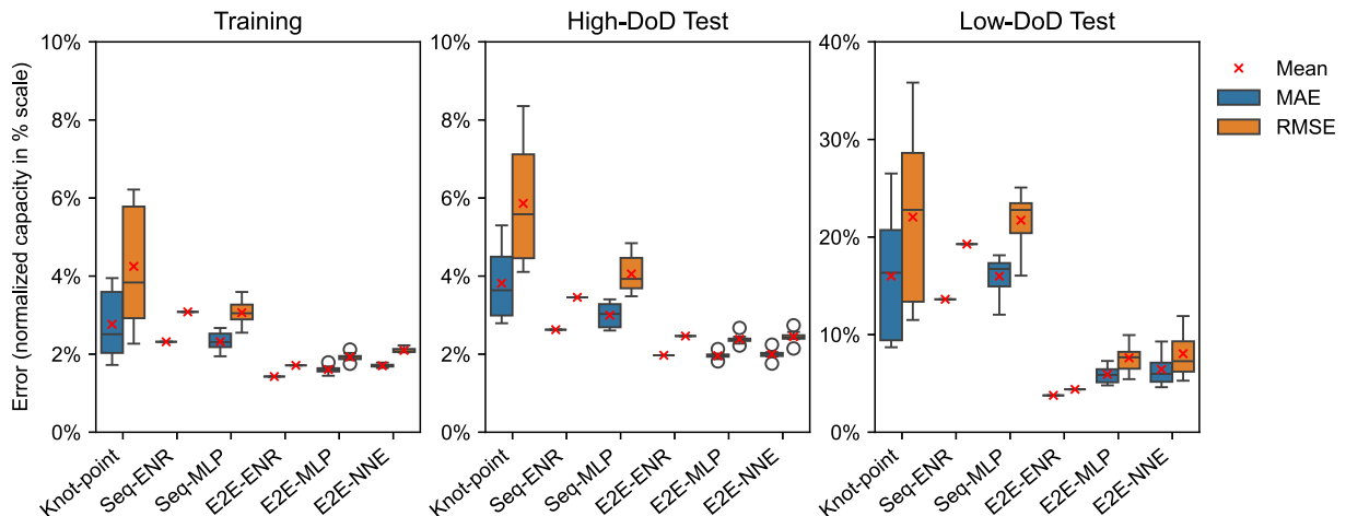
Fig. 7. Capacity trajectory prediction error of different empirical-model-informed methods for cells in three subsets. The red cross indicates the mean.
