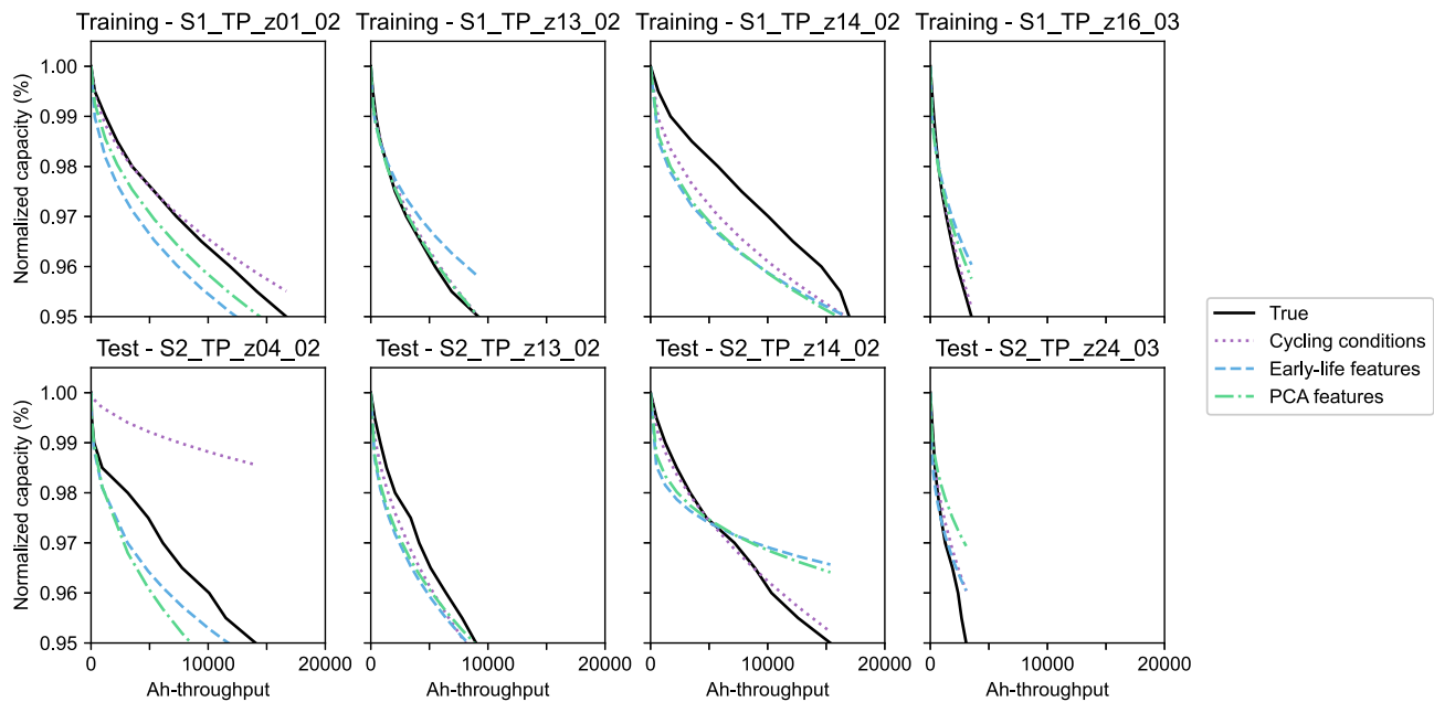
Fig. A.8. Predicted trajectories from E2E-ENR method for selected cells in the public NCA dataset.
