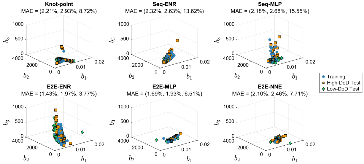
Fig. 8. Distribution of predicted empirical model parameters from six different methods. For MLP-based methods, the predicted parameters from one fold are visualized in this figure. The MAE values of trajectory predictions from a given distribution are listed in the parentheses for the training set, the high-DoD test set, and the low-DoD test set, respectively.
