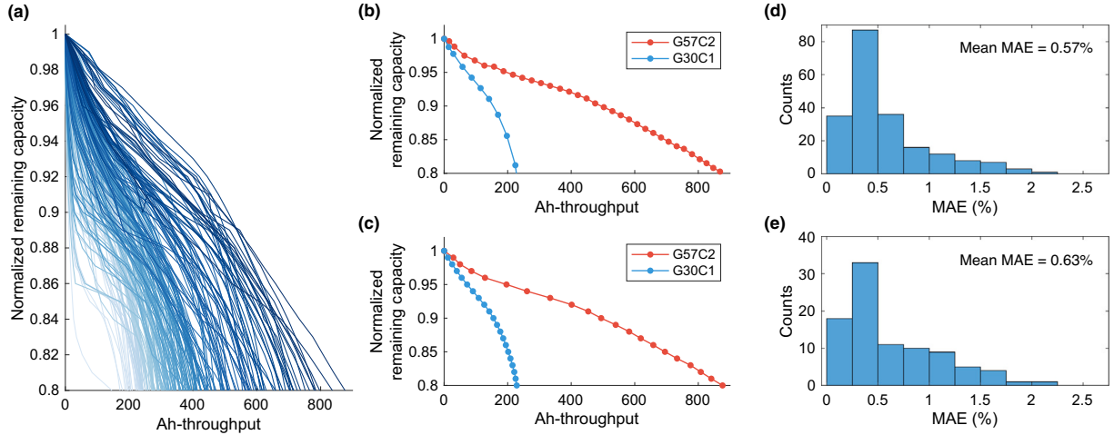
Fig. 3. Overview of the trajectory from cells in the dataset. (a) Capacity trajectories for all cells; (b) the data collected in RPTs for constructing the capacity trajectories for a long-life cell (G57C2) and a short-life cell (G30C1); (c) The capacity trajectories for the two cells on (b) constructed by interpolated data points using equidistant remaining capacity points; (d) An error histogram of fitting the empirical capacity fade model in Eq. (2) on the entire dataset; (e) An error histogram of fitting the empirical capacity fade model in Eq. (2) on the training set.
