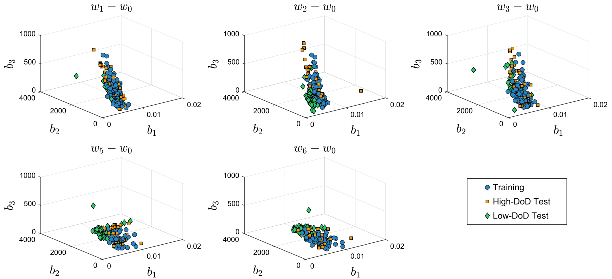
Fig. 12. Distribution of predicted empirical model parameters from five different RPT intervals for feature extraction using the E2E-ENR method.
