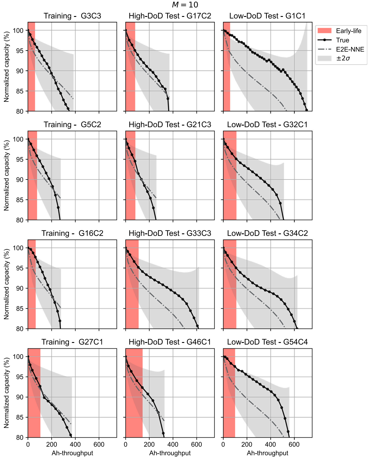
Fig. A.6. Predicted trajectories from E2E-NNE ( M = 10 ) for selected cells.
