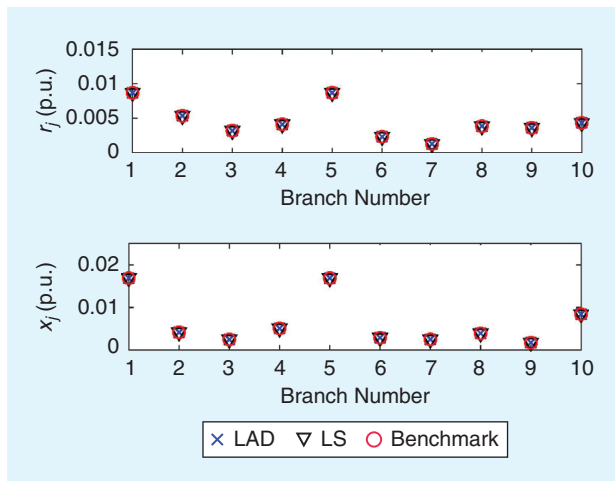
Figure 17. The results of line parameter estimation of a 13-bus test feeder. <AU: Kindly spell out p.u. so that the definition can be added to the caption.>
