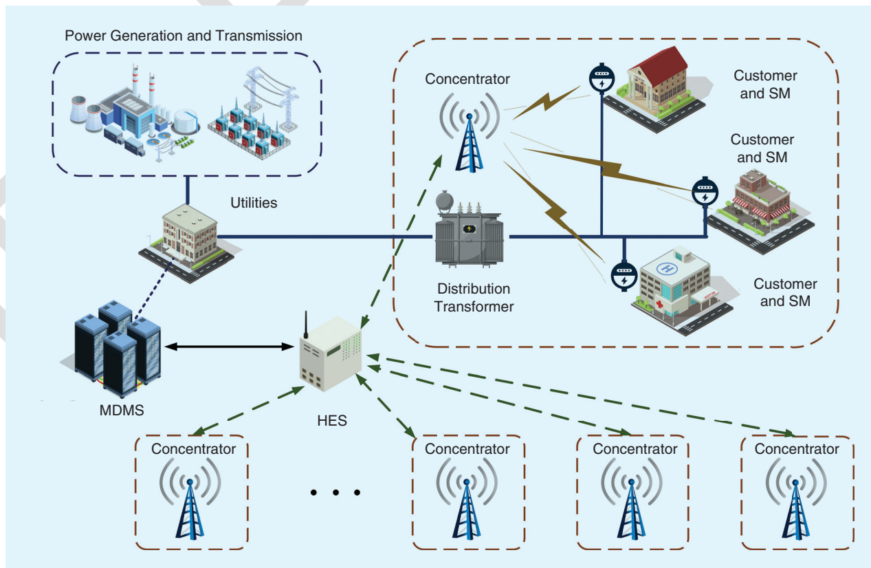
Figure 3. SM data collection and communication. HES: head-end system.
