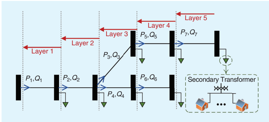
Figure 15. An example of a five-layer distribution network. <AU: Kindly spell out P and Q so that the definitions can be added to the caption.>
