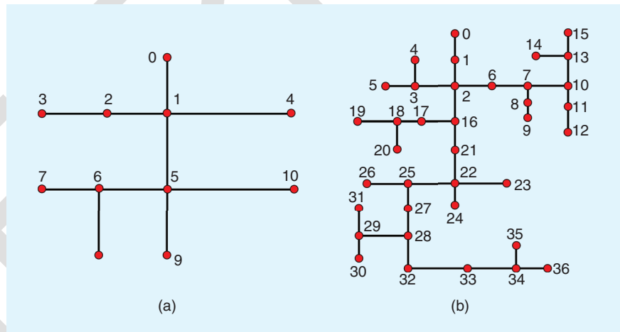
Figure 13. One-line diagrams of two test feeders: (a) IEEE modified 13-bus feeder and (b) IEEE 37-bus feeder.
