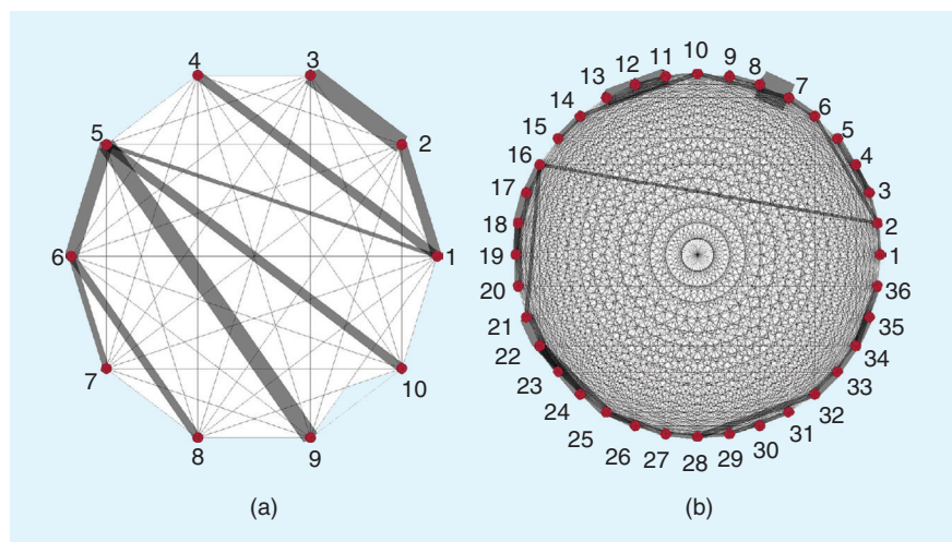
Figure 14. The estimated weighted Laplacian matrices of two test feeders using the proposed topology identification model: (a) IEEE modified 13-bus feeder and (b) IEEE 37-bus feeder.
