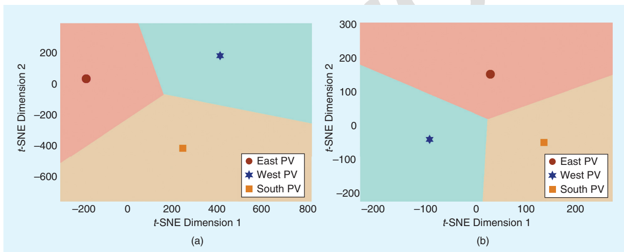
Figure 10. Visualizing the distinguishability of time-series PV generation curves of solar exemplars (a) hourly and (b) monthly. <AU: Kindly spell out t-SNE so that the definition can be added to the caption.>
